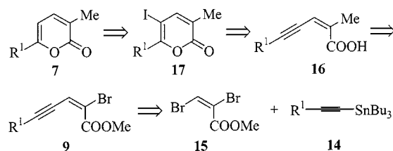
Scheme 4. Alternative retrosynthetic analysis of compounds 7
