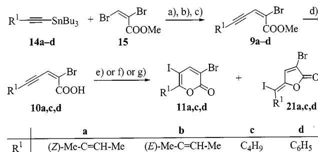
Scheme 6. Synthesis of 5-substituted ( E )-2-bromo-2-en-4-ynoic acids 10 and their iodolactonization; reagents: a) 14 (1.1 equiv.), PdCl 2 (PhCN) 2 (5 mol %), AsPh 3 (10 mol %), NMP, room temp., 20–24 h; b) 8 M aq. KF, Et 2 O; c) MPLC on silica gel; d) for compounds 9a,c,d : 1 M LiOH, THF, 24 h, then 10% H 2 SO 4 , 0 °C; e) Method A : I 2 (3.0 equiv.), NaHCO 3 (3.0 equiv.), MeCN, room temp., 1 h; f) Method B : ICl (1.0 equiv.), CH 2 Cl 2 , 0 °C, 1 h; g) Method C : NIS (1.1 equiv.), KHCO 3 (1.0 equiv.), MeCN, room temp., 1 h
