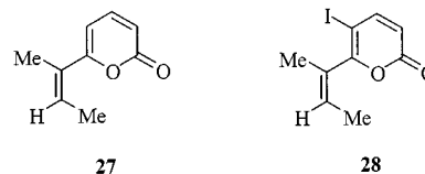
Figure 2. Chemical structures of compounds 27 and 28
