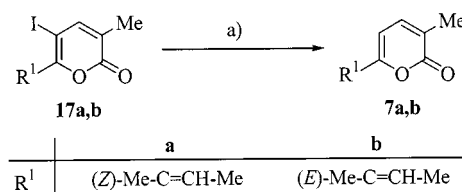
Scheme 10. Synthesis of stereoisomerically pure 7a and 7b ; reagents: a) Pd(OAc) 2 (2 mol %), Et 3 N (3.0 equiv.), PPh 3 (4 mol %), HCOOH (1.5 equiv.), DMF, 55–60 °C, 2–3 h
