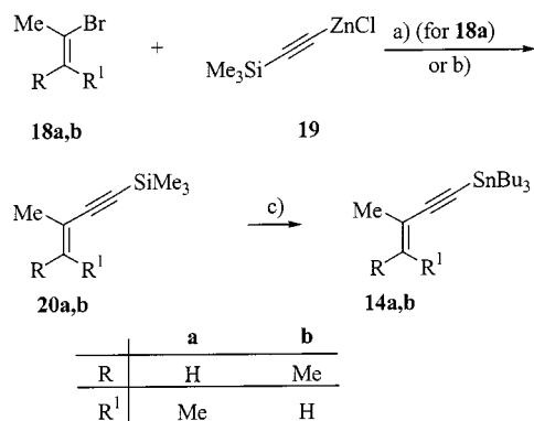
Scheme 5. Synthesis of ( Z )- and ( E )-3-methyl-3-penten-1-ynyltributyltin ( 14a ) and ( 14b ); reagents: a) 19 (1.25 equiv.), Pd(PPh 3 ) 4 (5 mol %), THF, 65 °C, 6 days; b) 19 (1.25 equiv.), Pd(PPh 3 ) 4 (5 mol %), THF and DMF (1:1), 60 °C, 24 h (for 18a ) and 3 h (for 18b ); c) (Bu 3 Sn) 2 O (0.47 equiv.), TBAF (0.02 equiv.), THF, 65 °C, 2.5 h
