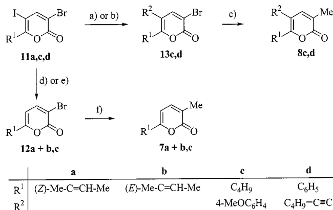
Scheme 8. Synthesis of 5,6-disubstituted 3-bromo-2(2 H )-pyranones 13 , 5,6-disubstituted 3-methyl-2(2 H )-pyranones 8 , 6-substituted 3-bromo-2(2 H )-pyranones 12 and 6-substituted 3-methyl-2(2 H )-pyranones 7 ; reagents: a) for 11c : 4-MeOC 6 H 4 SnBu 3 ( 24 ) (1.1 equiv.), PdCl 2 (PhCN) 2 (5 mol %), CuI (10 mol %), AsPh 3 (10 mol %), NMP, 23 h, 45 °C; b) for 11d : 14c (1.1 equiv.), PdCl 2 (PPh 3 ) 2 (3 mol %), THF, 22 h, 20 °C, then 44 h, 45 °C; c) Me 4 Sn (3.0 equiv.), PdCl 2 [P( o -tolyl) 3 ] 2 (5 mol %), CuI (10 mol %), NMP, 80 °C, 22 h; d) for 11a : Pd(OAc) 2 (2 mol %), Et 3 N (3.0 equiv.), PPh 3 (4 mol %), HCOOH (1.5 equiv.), DMF, 60 °C, 5 h; e) activated zinc dust (5.0 equiv.), THF, 2.5–13.5 h, then H 3 O + ; f) Me 4 Sn (3.0 equiv.), PdCl 2 [P( o -tolyl) 3 ] 2 (5 mol %), CuI (10 mol %), NMP, 80 °C, 22 h.
