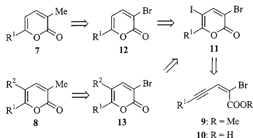
Scheme 3. Retrosynthetic analysis of compounds 7 and 8
