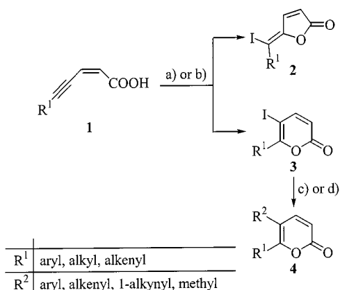
Scheme 1. Synthesis of 5,6-disubstituted 2( 2H )-pyranones; reagents: a) I 2 (3 equiv.), NaHCO 3 (3 equiv.), MeCN, 1.5 h, room temp.; b) ICl (1 equiv.), CH 2 Cl 2 , 1.5 h, room temp.; c) R 2 SnBu 3 or R 2 SnMe 3 (1.2–3.0 equiv.), NMP, PdCl 2 (PhCN) 2 (5 mol %), CuI (10 mol %), AsPh 3 (10 mol %), 20–80 °C, 22–80 h; d) R 2 SnBu 3 (1.2 equiv.), THF, PdCl 2 (PPh 3 ) 2 (3 mol %), 20–50 °C, 40–46 h
