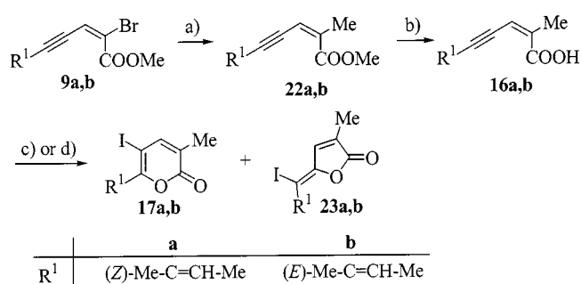
Scheme 7. Synthesis of 5-substituted ( Z )-2-methyl-2-en-4-ynoic acids 16 and their iodolactonization; reagents: a) Me 4 Sn (3.0 equiv.), PdCl 2 [P( o -tolyl) 3 ] 2 (5 mol %), CuI (10 mol %), NMP, 70 °C, 2.5 h; b) 1 M LiOH, THF, room temp., 24 h, then 10% H 2 SO 4 , 0 °C; c) Method A : I 2 (3.0 equiv.), NaHCO 3 (3.0 equiv.), MeCN, room temp., 1 h; d) Method B : ICl (1.0 equiv.), CH 2 Cl 2 , 0 °C, 1 h
