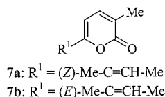
Figure 1. Chemical structures of compounds 7a and 7b
