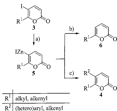
Scheme 2. Synthesis of 6-substituted and 5,6-disubstituted 2( 2H )-pyranones; reagents: a) activated zinc dust (3 equiv.), THF, room temp., 3–3.5 h; b) 5% HCl, 0 °C; c) R 2 X (X = Br, I) (0.83–1.43 equiv.), Pd 2 (dba) 3 (2 mol %), PPh 3 (8 mol %), THF, 20–70 °C; 15–63 h
