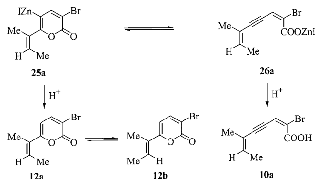
Scheme 9. Possible explanation for the formation of compounds 10a , 12a , and 12b in the reaction between 11a and activated zinc dust, followed by acidic hydrolysis
